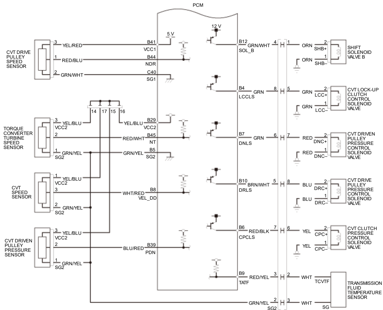
PCM Connector Terminal Locations
